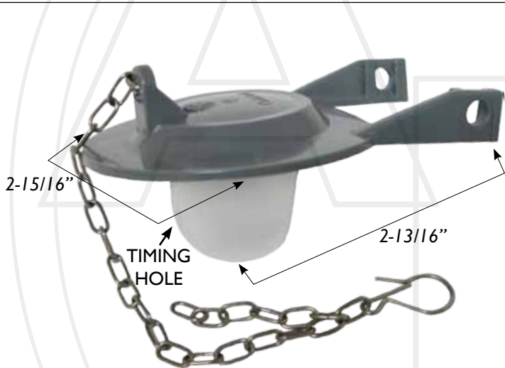
THU257 • FLAPPER CHAIN LENGTH (link w/clip): 7-1/2"
