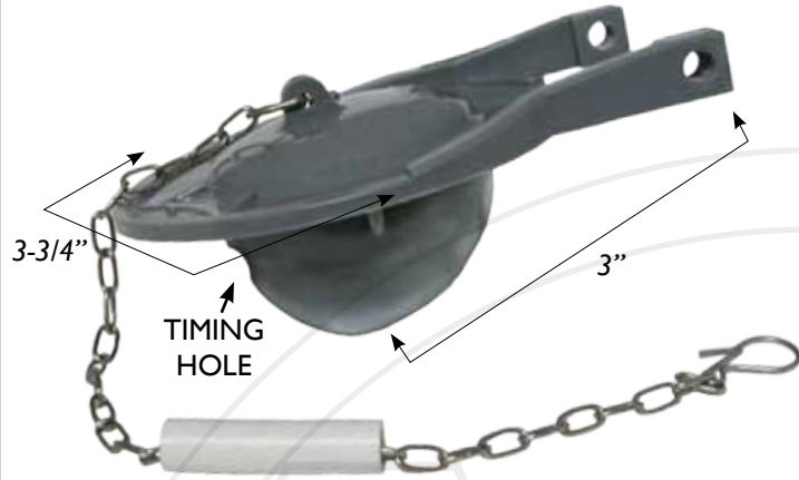
THU347S • EMAX & GMAX FLAPPER CHAIN LENGTH (link w/clip): 9"
