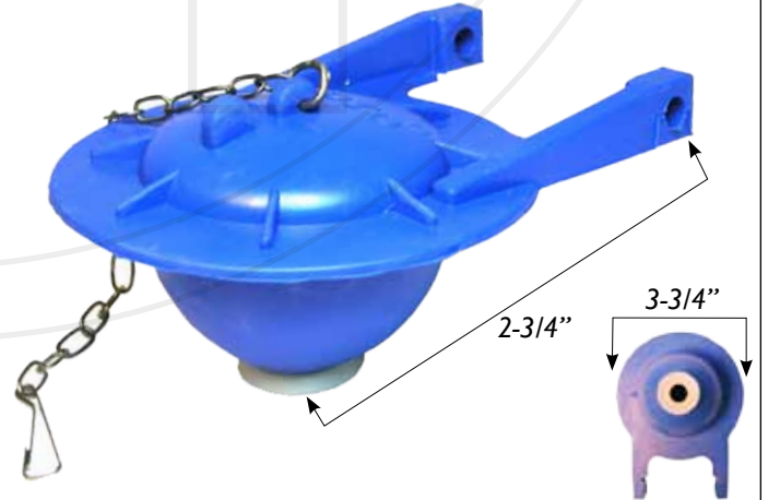
TUH140S • POWER GRAVITY FLAPPER CHAIN LENGTH (link w/clip): 6.5"
