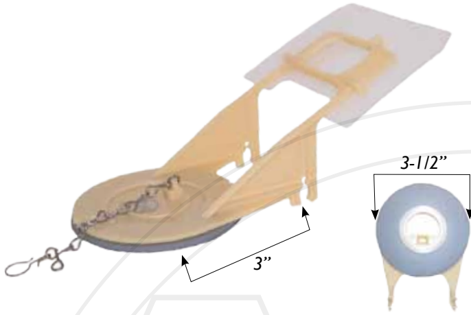
TUH092-5 • FLAPPER CHAIN LENGTH (link w/lj-clip): 3"
